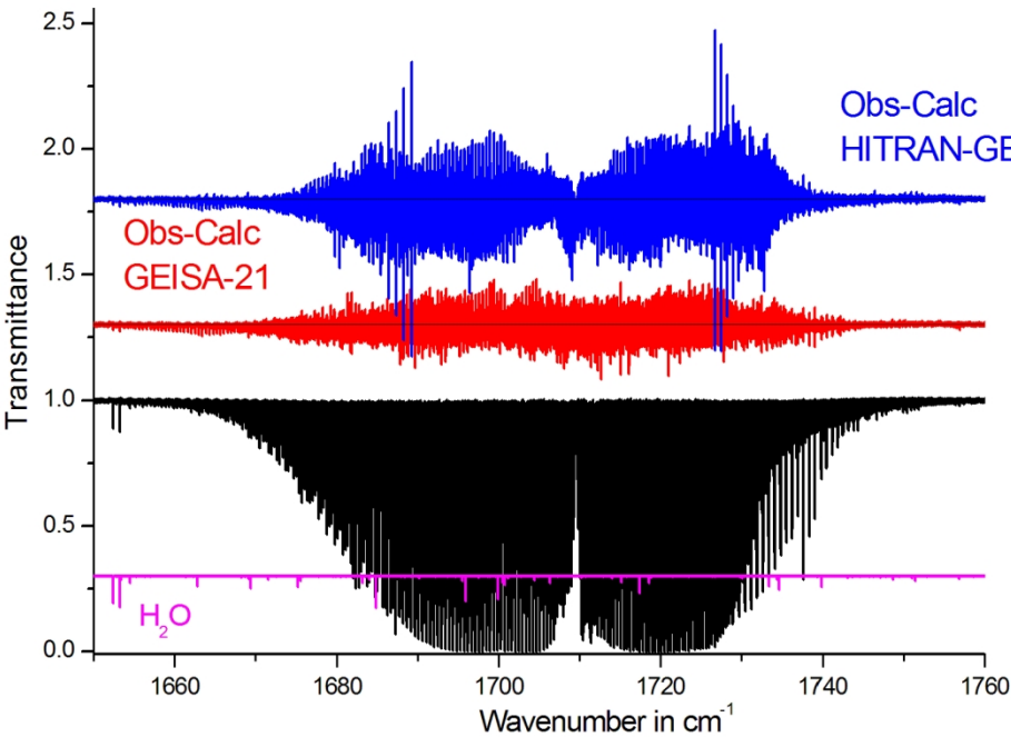
Overview of the HNO 3 spectrum recorded in the 5.8 μm region. The (Observed – Calculated) signals are compared for the old (HITRAN-GEISA) and new (GEISA-21) line lists. Both computations account for the presence of water vapour in the absorption cell.
