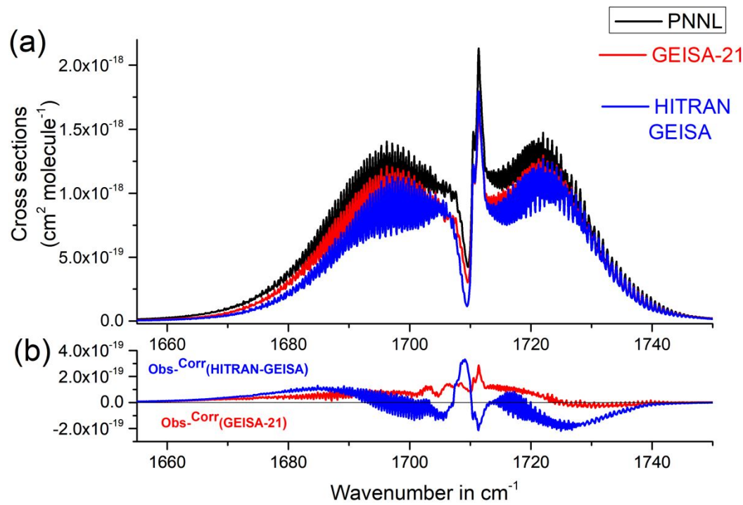
Fig. 4: (a) Comparison of the PNNL cross sections (in \text{cm}^2/\text{molecule} at 296K) with their corresponding values using the HITRAN-GEISA linelist and the GEISA-21 linelist. (b) (Observed – (corrected) calculated values) using HITRAN-GEISA and GEISA-21, when accounting for the missing hot bands: the HITRAN-GEISA and GEISA-21 computed cross sections are multiplied by \text{Factor}_{\text{Missing}}^{\text{HIT-GEISA}} = 1.30 and \text{Factor}_{\text{Missing}}^{\text{GEISA-21}} = 1.09 correcting factors, respectively.
