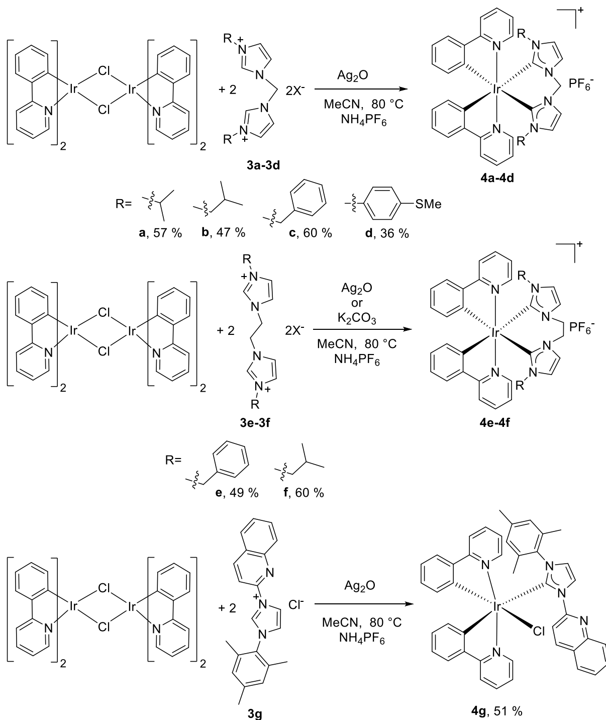
Scheme 2. Synthesis of cyclometalated iridium(III) NHC complexes 4a-4g .
