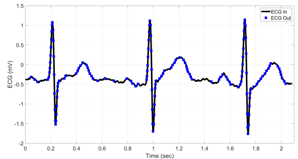
Fig. 2. Level-crossing sampling of ECG from the MIT-BIH dataset.
