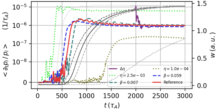
Figure 6: Dependence of the heating rate on the resistivity. In the run labeled \Delta\eta the resistivity is \eta = 2.5e - 03 up to t = 2000\tau_A , and it is then changed to the reference value \eta = 5.0e - 04 , thus showing a direct dependence of the heating on the resistivity. The simulation with lowest \eta = 1.0e - 04 did not reach saturation of the island in the time frame shown, as the heating saturates much earlier. In greyscale are the island sizes matching the simulations with the same line style.
