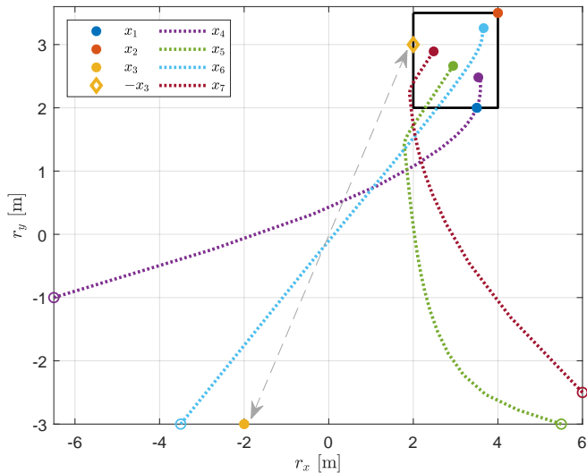
Fig. 3. Bipartite containment tracking of (25) with perturbation.
