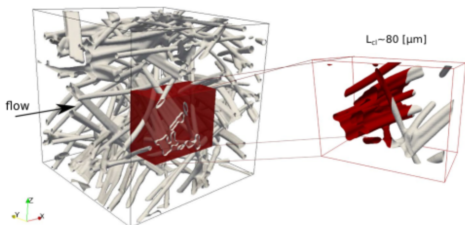
Fig. 15 Calcarb dataset characterized in this article, with a red box to highlight a small area that influences the behavior of the flow inside the whole domain
