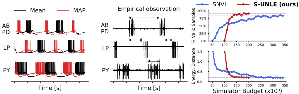
Figure 6: Performance of SUNLE using 100000 prior samples in the first round, followed by 10 rounds of 10000 samples. We observe a significant increase in the fraction of valid samples generated by the model.
