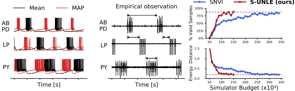
Figure 3: Inference SUNLE on a model of the crab’s pyloric network. Left: simulations obtained by using the final posterior mean and maximum a posteriori (MAP) as a parameter. Center: the empirical observation x_o : arrows indicate the summary statistics. Top-right: fraction of simulated observations with well-defined summary statistics (higher is better) at each round for SNVI and SUNLE, with dashed lines indicating the maximum fraction for each method. Bottom-right: performance of the posterior using the Energy Scoring Rule (lower is better).
