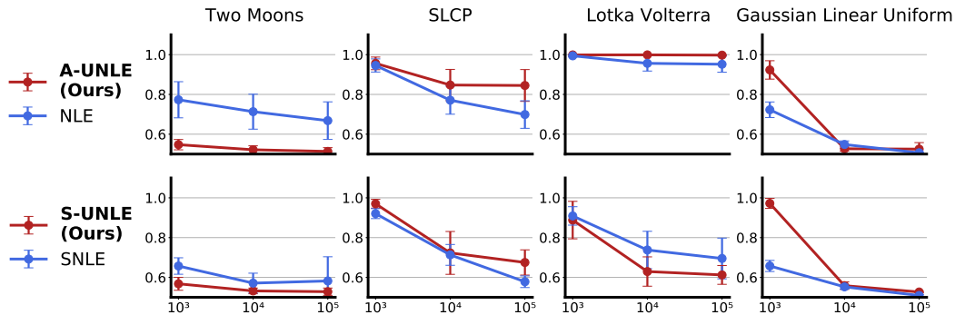
Figure 2: Performance of AUNLE (resp. SUNLE) compared with NLE (resp. SNLE), using the Classifier Accuracy Metric (Lueckmann et al., 2021) (lower is better). AUNLE and SUNLE exhibit robust performance across a wide array of problem and posterior structures.
