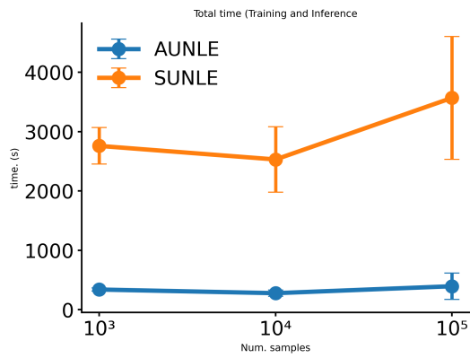
Figure 8: Compute time for A-UNLE and S-UNLE as a function of the number of samples.
