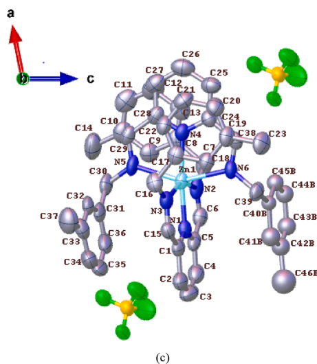
Fig. 4. Labelled ORTEP drawing of 1 (a) in a -axis and 2 (b) and 3 (c) in b -axis at 120 K. Thermal ellipsoids are drawn on 30% probability level. Hydrogen atoms and solvent molecules are omitted for clarity.
