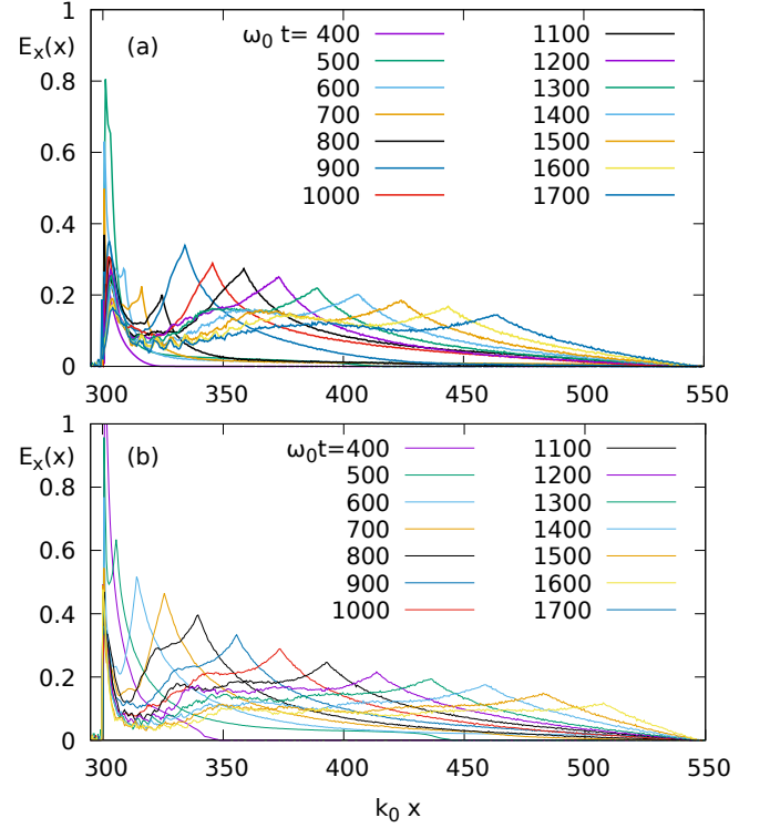
FIG. 18. Spatial profiles, in x , of the electric field eE_x/(m_e \omega_0 c) at the rear side of the target for a sequence of time instants (in steps of 100\omega_0^{-1} ), for the case of target thickness of 150k_0^{-1} , and for the cases with the gradient k_0 L_g = 0 (a, upper plot) and k_0 L_g = 3 (b, lower).
