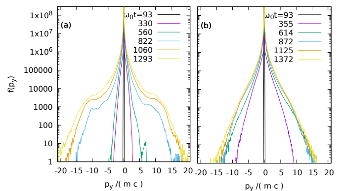
FIG. 11. Electron distribution density f(p_y) , at different time instants taken in the bulk of the plasma ( 130 < k_0 x < 230 ), as a function of the electron momenta p_y/(m_e c) . (a), left : for a profile with a step-like density profile ( k_0 L_g = 0 ); (b), right : for a density profile with a gradient between n_e = 0 and n_e = 100n_c around x = x_c (i.e. k_0 L_g = 3 ).
