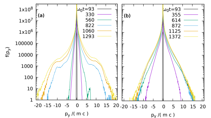
FIG. 11. Electron distribution density f(p_y) , at different time instants taken in the bulk of the plasma ( 180 < k_0 x < 280 ), as a function of the electron momentum p_y/(m_e c) . (a), left : for a profile with a step-like density profile ( k_0 L_g = 0 ); (b), right : for a density profile with a gradient between n_e = 0 and n_e = 100n_c around x = x_c (i.e. k_0 L_g = 3 ).
