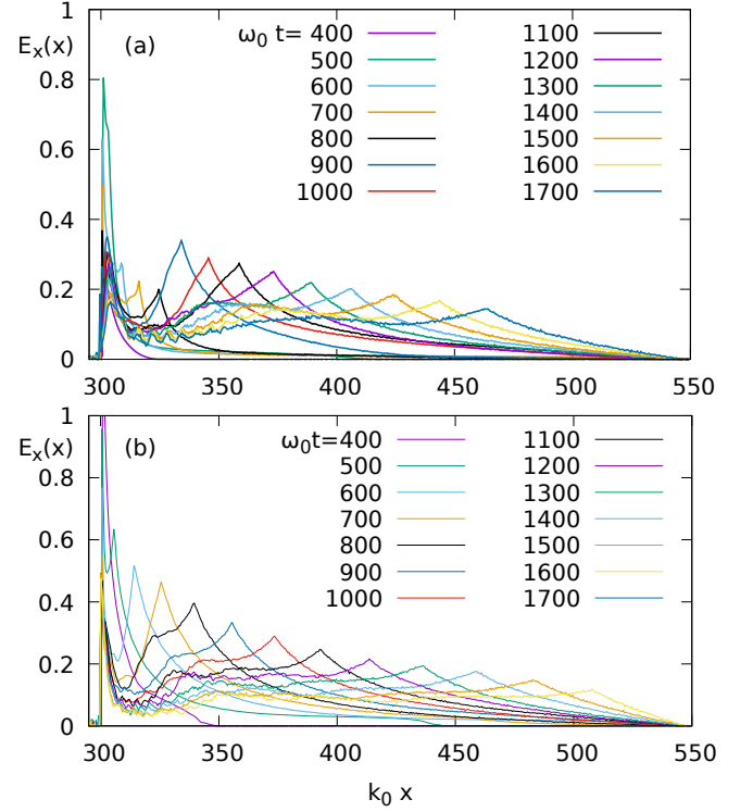
FIG. 18. Spatial profiles, in x , of the electric field eE_x/(m_e \omega_0 c) at the rear side of the target for a sequence of time instants (in steps of 100\omega_0^{-1} ), for the case of target thickness of 150k_0^{-1} , and for the cases with the gradient k_0 L_g = 0 (a, upper plot) and k_0 L_g = 3 (b, lower).
