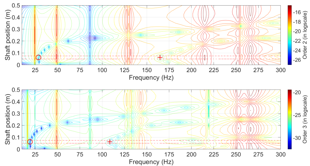
Figure 7. Case 3—Identification of the crack location based on the antiresonances of orders 2 and 3 (results are drawn for the vertical amplitudes in log-scale).
