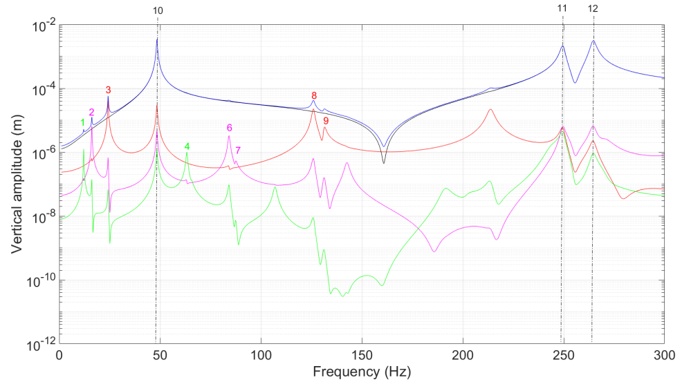
Figure 2. Vertical amplitudes at 0.1 m from the left side of the rotor system with a breathing crack (case 1— \mu = 1 and L_{crack} = 0.3625 m from the left side) (blue = nonlinear response, black = order 1, red = order 2, magenta = order 3, green = order 4).
