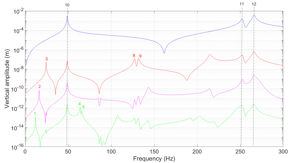
Figure 4. Vertical amplitudes at 0.1 m from the left side of the rotor system with a breathing crack (case 3— \mu = 0.1 and L_{crack} = 0.0625 m from the left side) (blue = nonlinear response, black = order 1, red = order 2, magenta = order 3, green = order 4).
