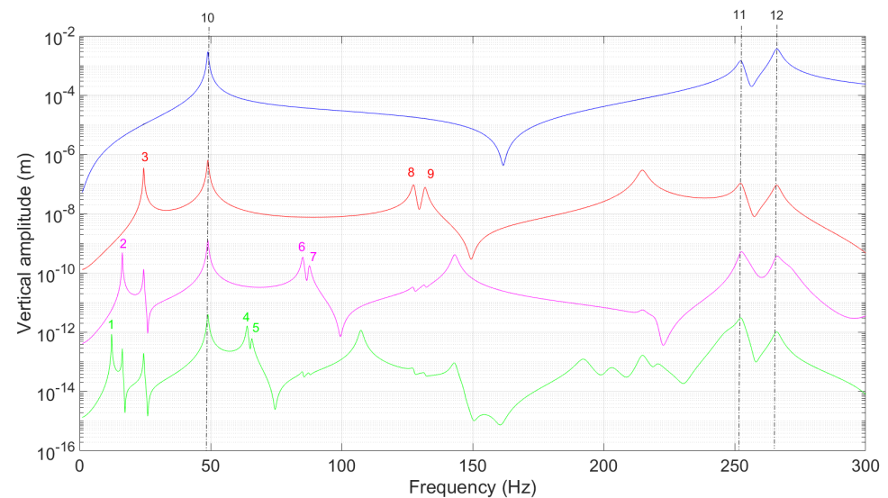
Figure 3. Vertical amplitudes at 0.1 m from the left side of the rotor system with a breathing crack (case 2— \mu = 0.1 and L_{crack} = 0.2625 m from the left side) (blue = nonlinear response, black = order 1, red = order 2, magenta = order 3, green = order 4).
