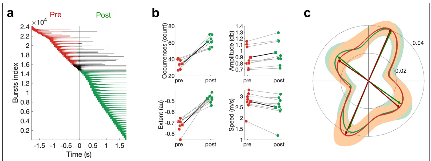
Figure 5. Differences in pre- and post-movement beta bursts. (a) Burst timing relative to the button press across all subjects. Each horizontal line represents one burst. Bursts are sorted by burst onset and burst duration using multiple-level sorting, yielding the burst index. Pre-movement bursts (i.e. bursts that start and end prior to the button press) are highlighted in red, post-movement bursts (i.e. bursts that start after the button press) are highlighted in green, and bursts that start prior to the button press and end after the button press are highlighted in black. (b) Number of bursts, burst amplitude, burst extent, and burst speed differ between pre- and post-movement bursts. Medians are shown for each subject (circles) and the mean across the subjects' medians (squares). (c) Propagation direction does not differ between pre- and post-movement bursts. Shown are polar probability histograms separately for pre- and post-movement bursts. Probability distributions were calculated for each subject individually and then averaged (dark line, N=8 ). Variability across subjects is expressed as standard deviation from the mean (light area). Von Mises functions were fitted separately for pre- and post-movement bursts.
