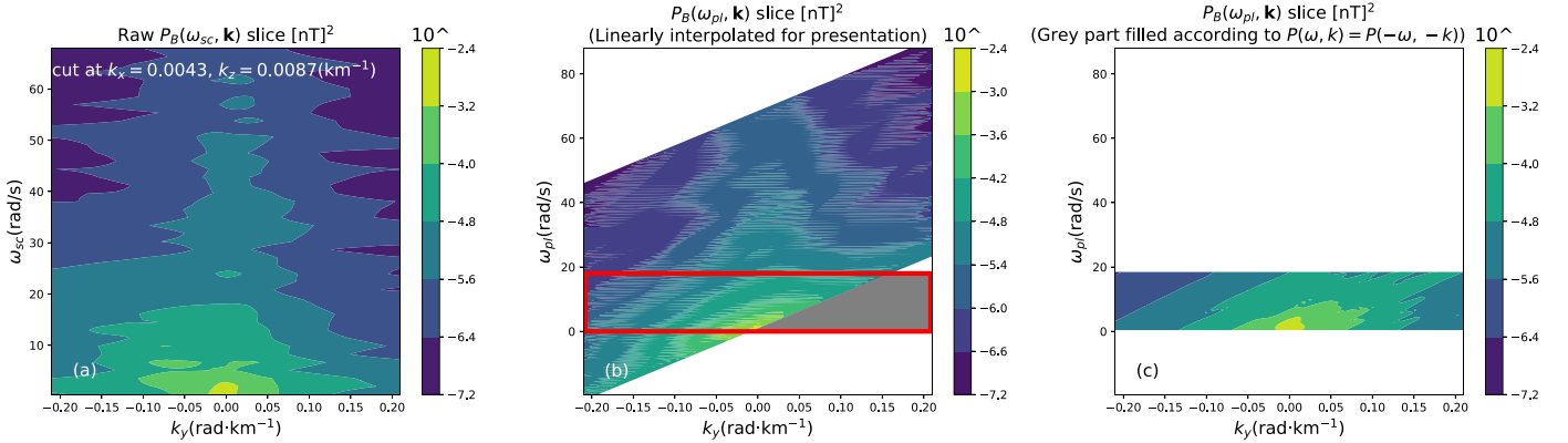
Figure 5. Cuts of energy distribution in the \omega-k plane. The angular frequencies are (a) in the spacecraft frame and (b) in the plasma frame obtained by the Doppler relation. Panel (c) shows a result after filling the gray part in panel (b) with its mirror counterpart.
