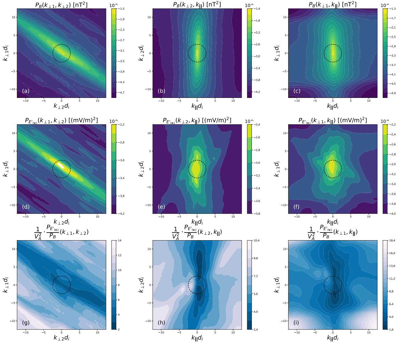
Figure 2. (a–f): reduced 2D distributions of \text{PSD}_B(\omega_{\text{pl}}, \mathbf{k}) and \text{PSD}_{E'_{(v_i)}}(\omega_{\text{pl}}, \mathbf{k}) , where P(k_{\parallel}, k_{\perp 1}) = \iint \text{PSD}(\omega_{\text{pl}}, \mathbf{k}) dk_{\perp 2} d\omega_{\text{pl}} , and so forth. (g–i): P_{E'_{(v_i)}}/P_B , normalized by the square of the Alfvén speed, V_A^2 , plotted to present the detail of the spectral bifurcation between P_B and P_{E'_{(v_i)}} . The black dashed circles centered at (0,0) with a length of k_{\min} denote a region within which there is large uncertainty.
