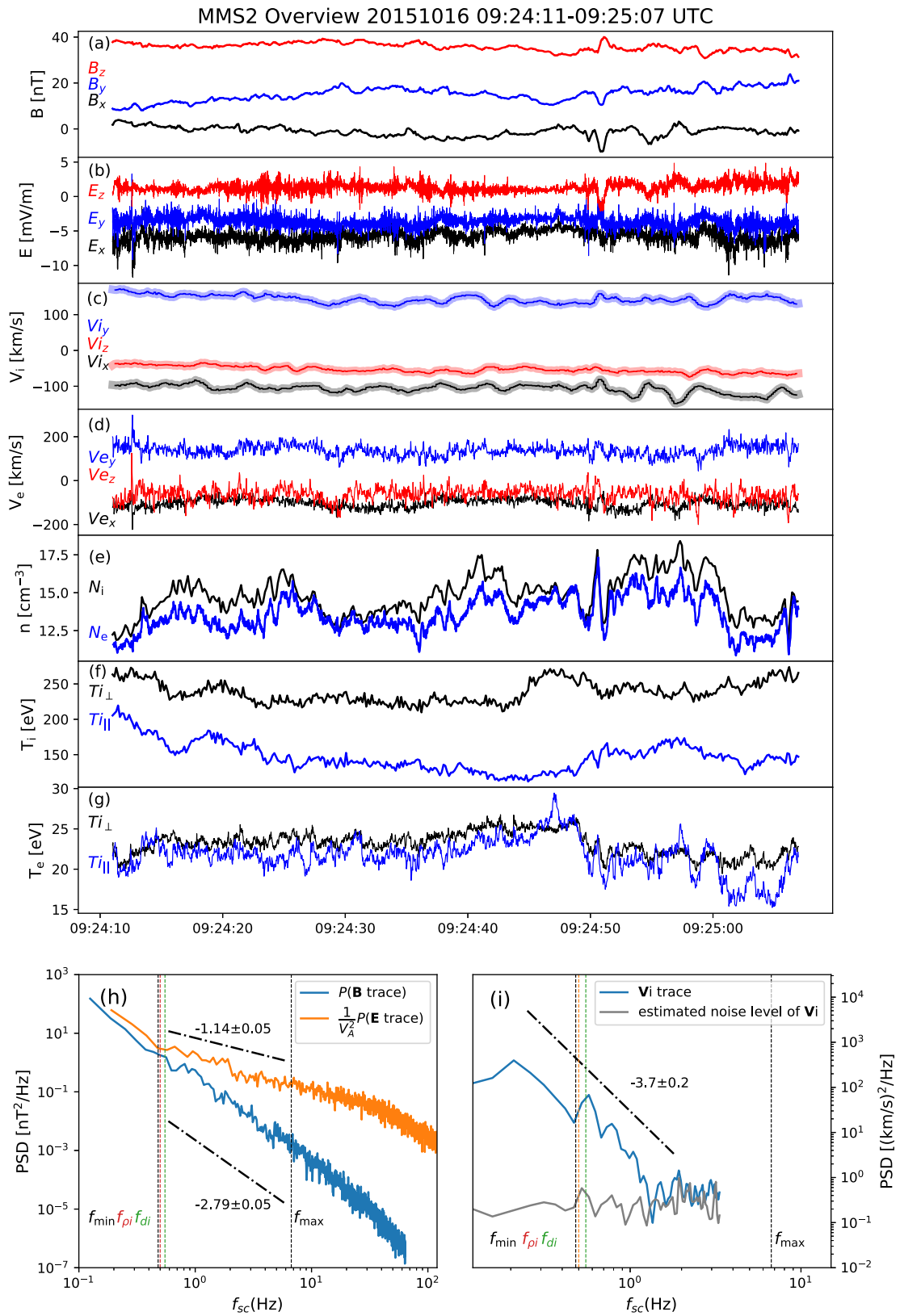
Figure 1. Time series of the MMS2 observations in GSE coordinates of (a) the magnetic field, (b) the electric field, (c, d) the velocities of the electrons and ions, where the wider background lines denote the measurements and the thinner lines are the resampled data, (e) the ion number density, (f, g) the temperature of the ions and electrons, (h) power spectra of the measured magnetic and electric fluctuations, and (i) power spectrum of the measured ion-velocity fluctuations together with the noise level estimated with the method by Gershman et al. (2018). During the time interval, the directions of the background magnetic field and bulk flow of particles stayed nearly stationary. The power of the electric field fluctuations is normalized by the Alfvén speed. A sliding Hamming window is applied to the time sequences before calculating the power spectral densities.
