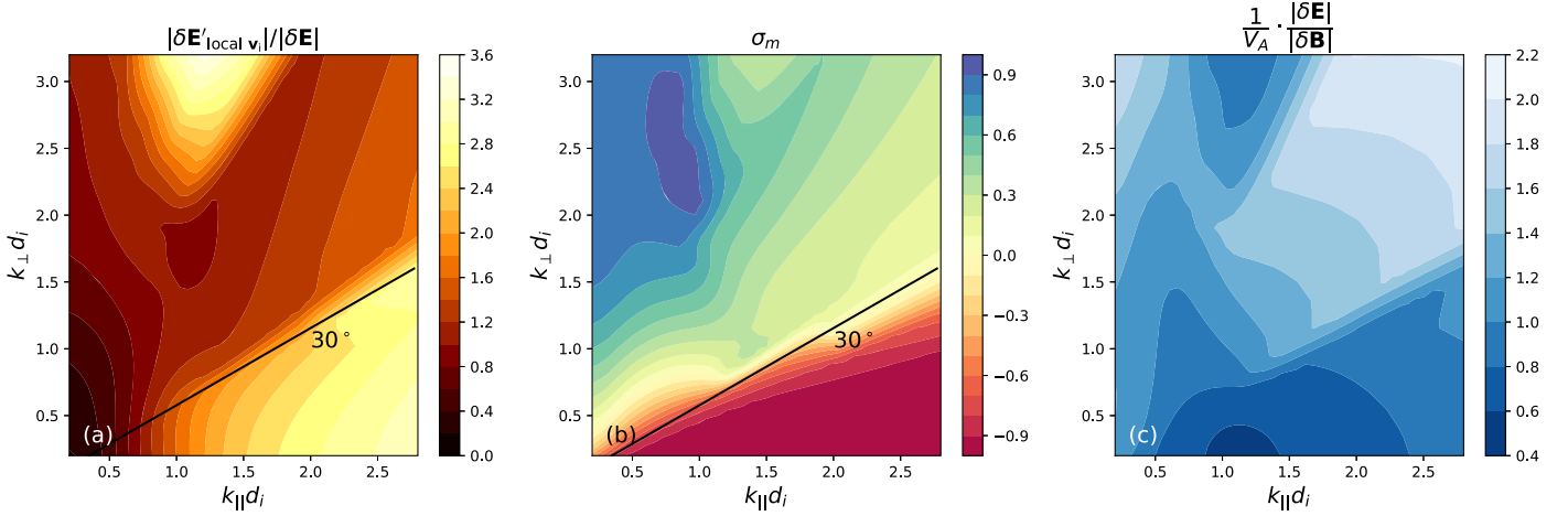
Figure 4. Metric of ion demagnetization/diffusion (left), normalized magnetic helicity (middle), and metric of dispersion computed by NHDS. The black line denotes \theta_{kB} \sim 30^\circ .
