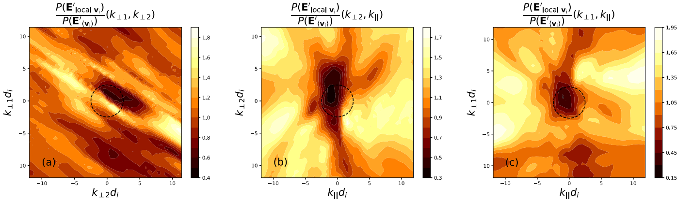
Figure 3. P_{E'_{\text{local } \mathbf{v}_i}}/P_{E'_{(\mathbf{v}_i)}} of the event, where P denotes PSD integrated over \omega_{\text{pl}} and different components of \mathbf{k} as defined in Figure 2. P_{E'_{\text{local } \mathbf{v}_i}}/P_{E'_{(\mathbf{v}_i)}} ( k_{\parallel}, k_{\perp} ) = \left(\iint \text{PSD}_{E'_{\text{local } \mathbf{v}_i}}(\omega_{\text{pl}}, \mathbf{k}) dk_{\perp,2} d\omega_{\text{pl}}\right) / \left(\iint \text{PSD}_{E'_{(\mathbf{v}_i)}}(\omega_{\text{pl}}, \mathbf{k}) dk_{\perp,2} d\omega_{\text{pl}}\right) . The black dashed circles centered at (0,0) with the length k_{\text{min}} denote a region within which there is large uncertainty.
