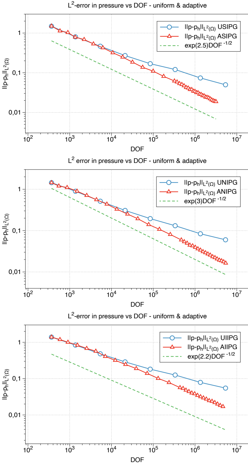
Fig. 5: Pressure L^2 -error vs. DOF for SIPG (up), NIPG (center) and IIPG (bottom).
