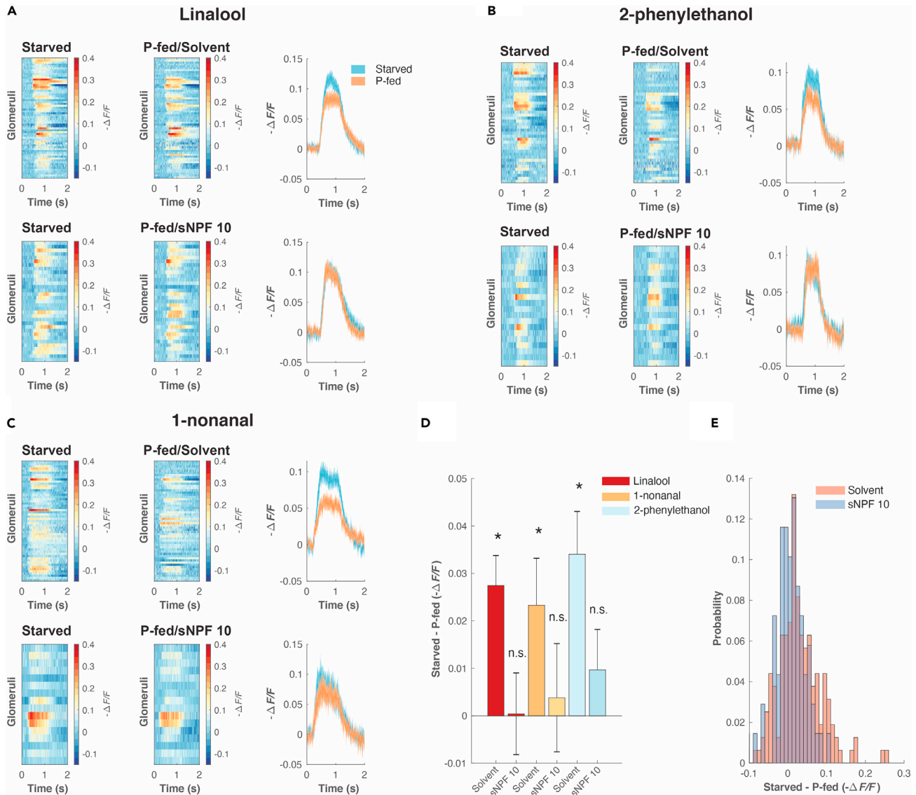
Figure 4. The effect of feeding status and sNPF on glomerular activity in the antennal lobe
