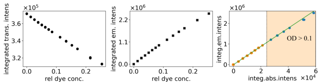
Figure S7. Spectrally-integrated transmitted and emitted light intensities (380 nm LED excitaion) as a function of quinine bisulfate concentration in 0.1M \text{HClO}_4(\text{aq}) (left and center columns), and the linearity (and slight loss of linearity) of the plot of the integral emitted light intensity vs the integral absorbed light intensity (right column).
