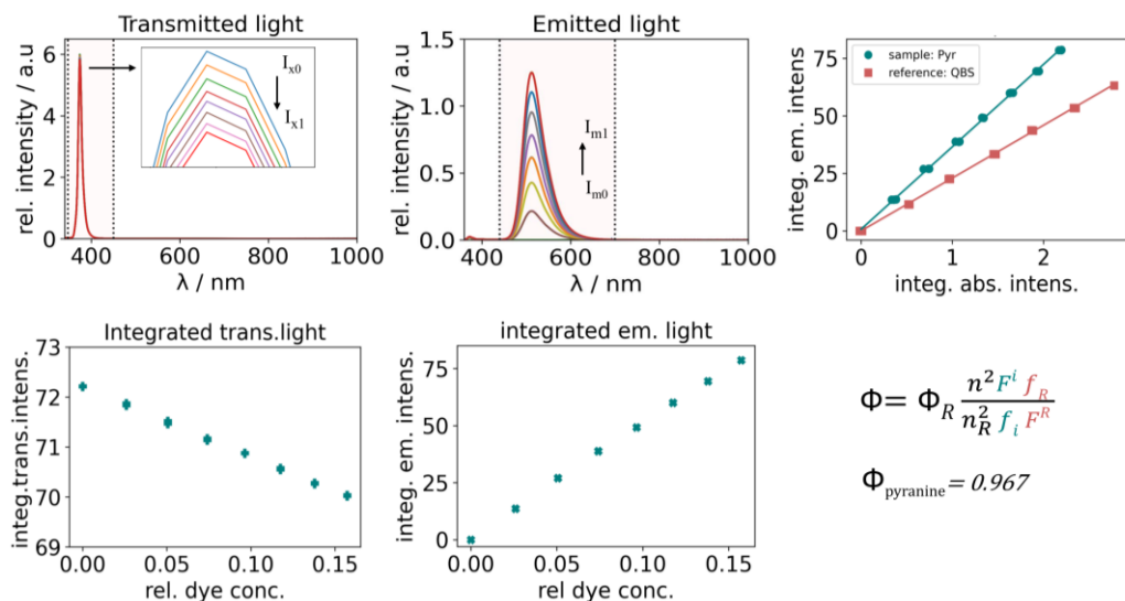
Figure 2. SAFER measurement of the PLQY of pyranine in 0.01M NaOH (aq) using QBS in 0.1M HClO 4(aq) as a reference. Only the spectra of the pyranine sample are shown. Left column: corrected transmitted light spectra and integrated intensities at increasing dye concentration. Center column: corrected emitted light spectra and integrated intensities. The limits of integration are shown as dotted vertical lines. Right column: plots of integrated emitted light vs absorbed light intensities for sample and reference, with the determination of PLQY via Eqn. (7). The value given in the figure is for the particular single measurement shown in the graphs. From four independent measurements, we obtained \Phi_{\text{pyranine}} = 0.96 \pm 0.08
