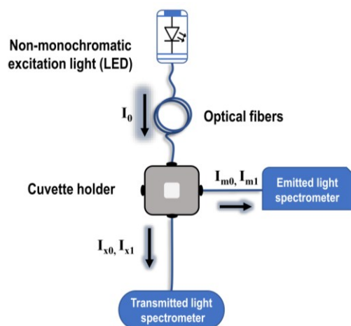
Figure 1. Set-up used for simultaneous light absorption and fluorescence emission measurements of limpid liquid samples for the determination of photoluminescence quantum yields
