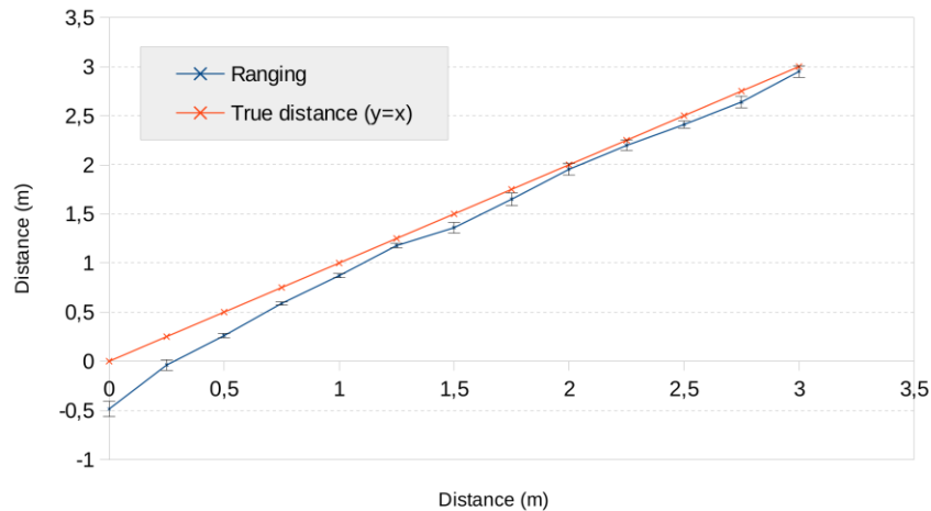
Figure 5. Ranging error.
