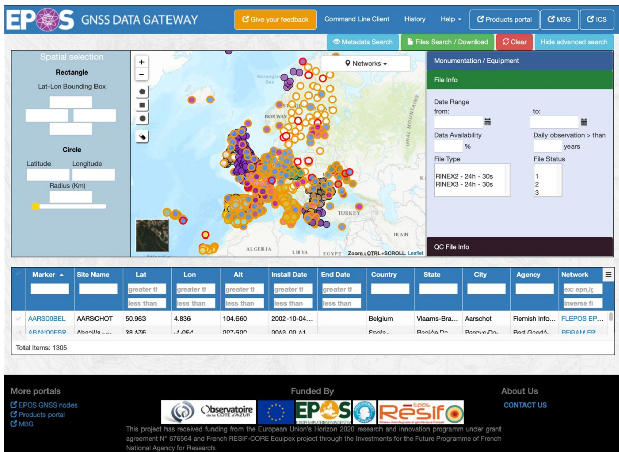
Figure 5. Web client of the EPOS-GNSS Data Gateway, one of the three available ways to discover and access the EPOS-GNSS metadata and data.
