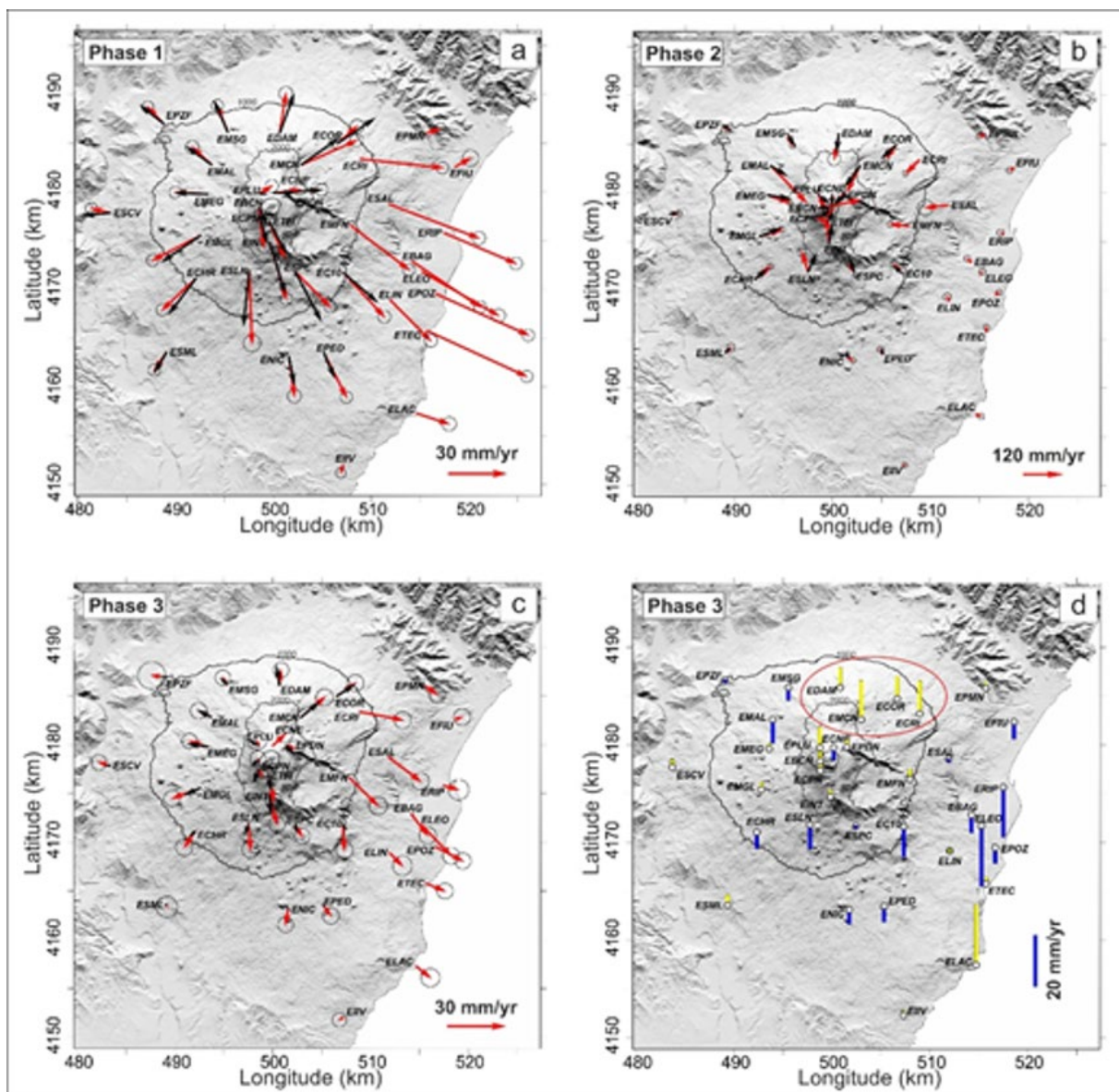
Figure 19. Recorded (red and grey arrows) and modelled (black arrows) horizontal CGPS velocity fields for the phases: (a) 26 April 2012-14 February 2013, (b) 15 February 2013-30 April 2013, (c) 20 May 2013-25 October 2013. Grey arrows were not considered in the modelling. (d) Vertical velocities (yellow rectangles for positive values and blue ones for negative values) for the third phase (20 May 2013-25 October 2013). The red circle highlights the CORS stations in the NE sector of Mt. Etna that show the anomalous ground deformation pattern.
