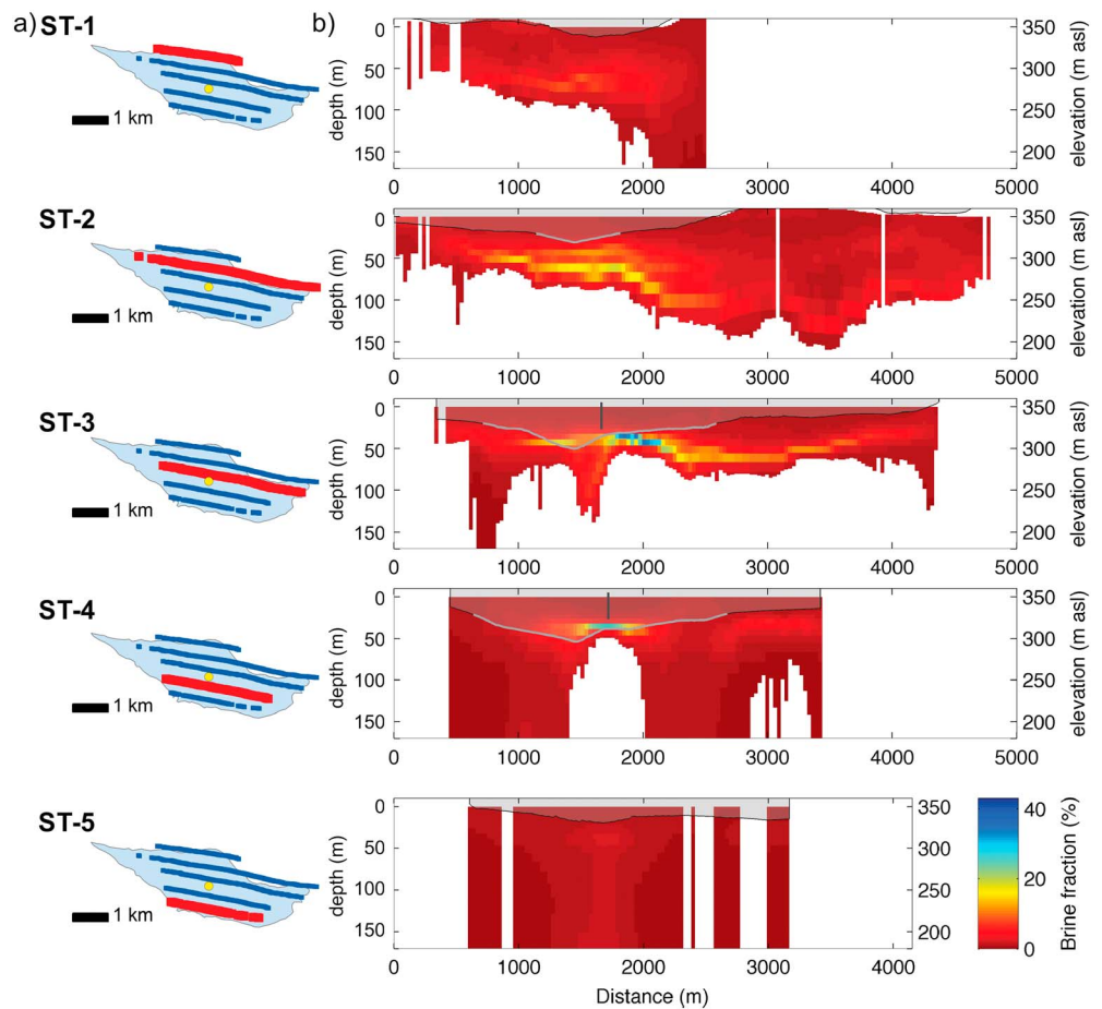
Figure 4. (a) Location of AEM flight lines on Lake Vida. The 2010 Lake Vida drill site is shown as a yellow dot between ST3 and ST4. (b) Brine fraction estimated from Archie’s law with a cementation factor of m = 2 . The black and grey lines superimposed on the profiles are known and estimated bathymetric depths, respectively. The area above this line represents the lake ice. The grey rectangle in ST3 and ST4 is the nearest approximate location and depth of the 2010 Lake Vida drill hole.
