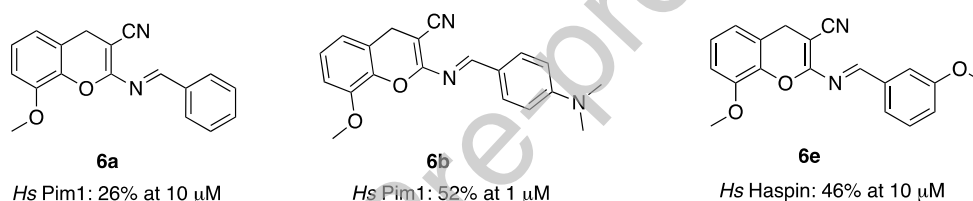
Figure 3: 2-Benzylideneamino-8-methoxy-4 H -chromene-3-carbonitrile 6(a,b) and 6e which are bioactive against protein kinases Pim1 and Haspin. Hs , Homo sapiens .
