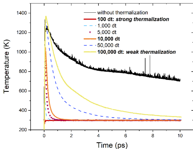
Figure 4- Comparison of different thermalization velocities of water.
