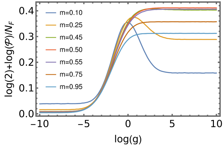
Figure 6: Reduced purity as a function of the dissipation strength g for seven different values of m = 0.10 – 0.95 , as given by Eq. (53). These results were obtained by exact diagonalization, with the correlation matrix obtained by the method described in Appendix E, for N_F = 60 and by averaging over 400 different realizations.
