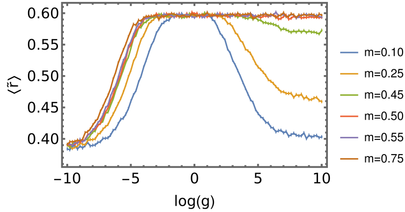
Figure 7: Mean level-spacing ratio \langle \tilde{r} \rangle as a function of the dissipation strength g for six different values of m = 0.1 – 0.75 . These results were obtained by exact diagonalization, with the correlation matrix obtained by the method described in Appendix E, for N_F = 60 and by averaging over 400 different realizations.
