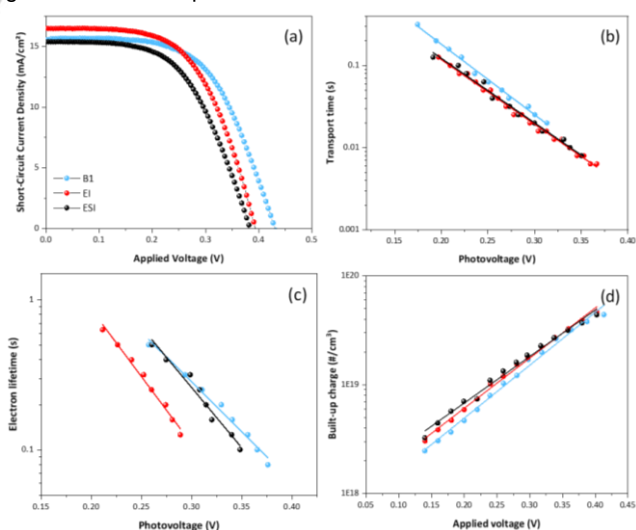
Figure 6. (a) J-V curve evolution of TB207 -based DSSC with different electrolytes: B ( \text{I}_3^-/\text{I}_2\text{Br} )/ ( \text{I}^-/\text{Br}^- ) in blue, E1 \text{I}_3^-/\text{I}^- in red, and ESI in black. (b) IMPS, (c) IMVS, and (d) dark charge extraction measurements on TB207 -DSSC are presented with the different electrolytes.
