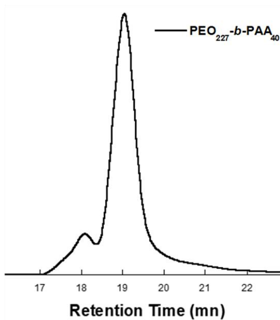
Figure S9.1.c Characterization of PEO- b -PAA by SEC-DMF after methylation of PAA with trimethylsilyl diazomethane. A molar mass in number M_n = 16\,526\text{ g}\cdot\text{mol}^{-1} was determined with calibration with PMMA standards. Typical sample concentration at 10\text{ mg}\cdot\text{mL}^{-1} . Solvent: DMF with 0.1 wt.% of LiBr as eluant and toluene as flux marker, flow: 0.8\text{ mL}\cdot\text{min}^{-1} . System Agilent technology: two columns PL1113-6300 respire 300 \times 7.5\text{ mm} and three detectors: refractive index PL0390-0601, two angles 15^\circ and 90^\circ light scattering and capillary viscometer PL0390-06034.
