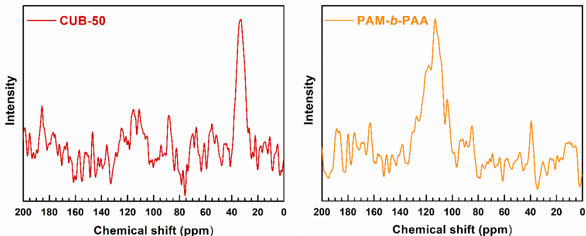
Fig. S2b: ^{15}\text{N} CP-MAS NMR spectra of (right) PAM- b -PAA and (left) hybrid mesoPIC materials CUB-50 prepared with 50% of PAM- b -PAA.
