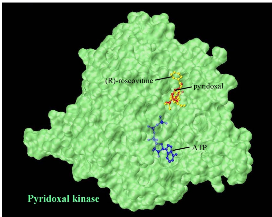
FIG. 8. Superimposition of the crystal structures of PDXK in complex with ( R )-roscovitine, an ATP analog or pyridoxal. The overall view of PDXK (green) shows that ( R )-roscovitine (yellow) binds at the site of pyridoxal (red) rather than at the site of ATP (blue).
