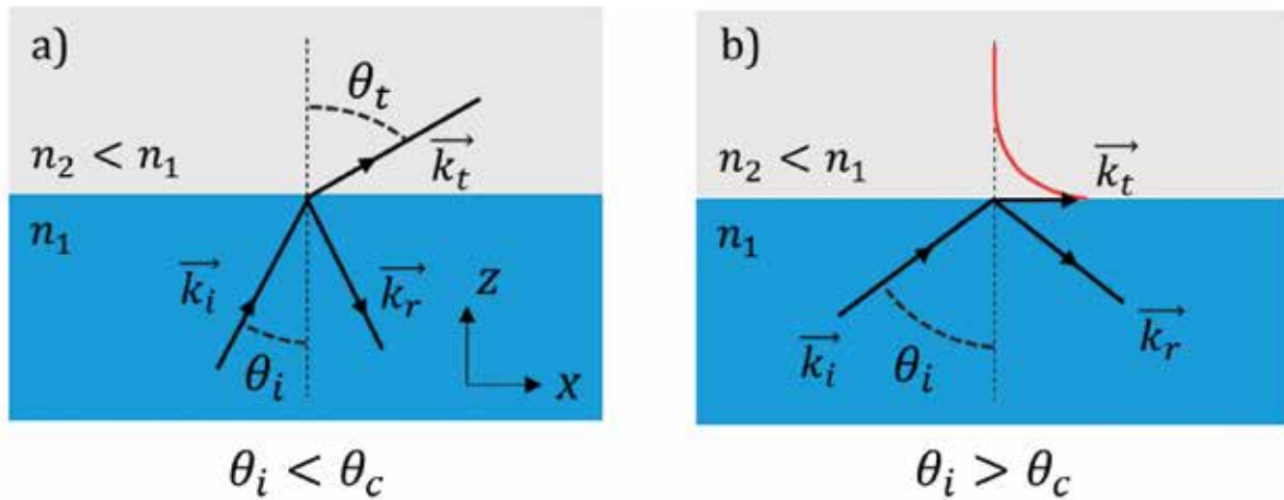
Figure a) Reflection and transmission at an optical interface for an oblique incidence below the critical angle. Figure b) Surface wave generation for an oblique incidence above the critical angle.
