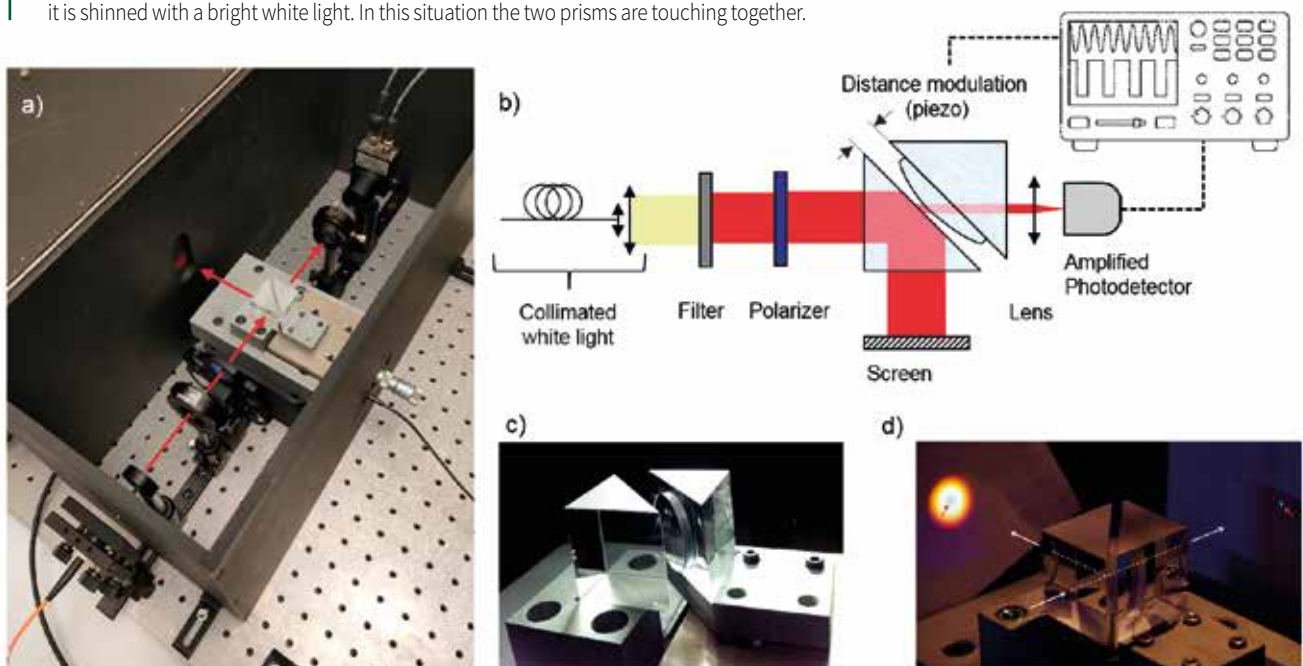
Figure 2. a) Picture of the turn-key setup for evidencing the frustrated total internal reflection. b) Schematic drawing of the experiment. c) Picture of the two prisms with the high radius of curvature lens glued on top of. d) Smartphone picture of the operating experiment once it is shined with a bright white light. In this situation the two prisms are touching together.
