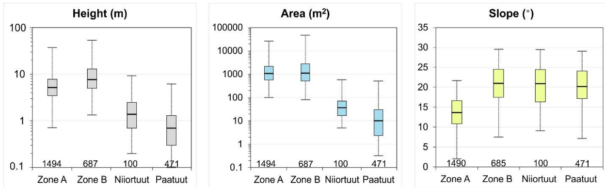
Figure 10 - Boxplots of the height, area, and flank slopes of the mounds in Zone A and Zone B of Hale Crater, Mars, and of mounds in Niortuut and Paatuut, Greenland; note that the vertical axes for height and area use a logarithmic scale. The whiskers show the maximum and minimum values, the boxes mark the interquartile range, and the thick horizontal black lines are the medians of each population. The numbers on the x-axis show the number of mounds in each population.
