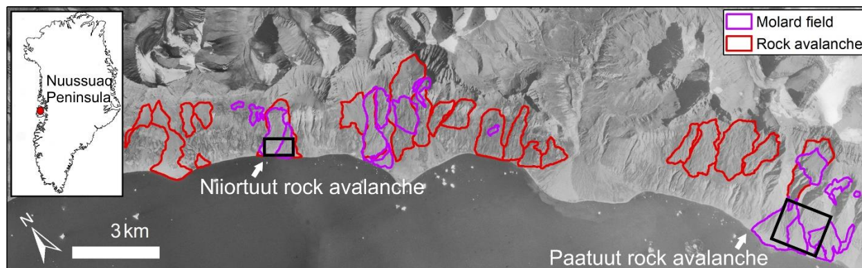
Figure 3 -The south-western slope of Nuussuaq Peninsula, showing the rock avalanches and molard field boundaries identified by field and airborne map observations. The black squares indicate the studied areas of Paatuut and Niortuut rock avalanches. The basemap is vertical aerial photographs of the south coast of Nuussuaq Peninsula from 1985, available from SDFI (The Danish Agency for Data Supply and Infrastructure). Inset map shows the location of the study area within western Greenland.
