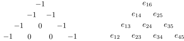
Fig. 3: The Shi vector of t in A_4 . The right triangle gives the coordinates of the Shi vector.
