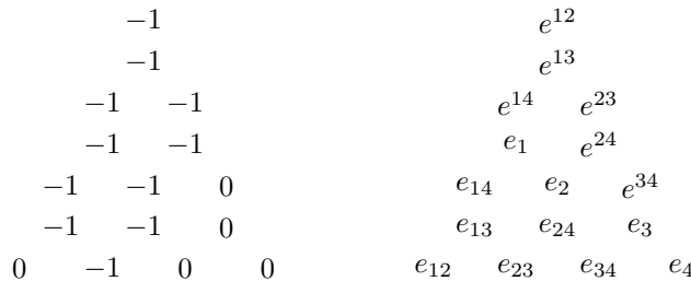
Fig. 5: The Shi vector of t in B_4 . The right part gives the coordinates of the Shi vector.
