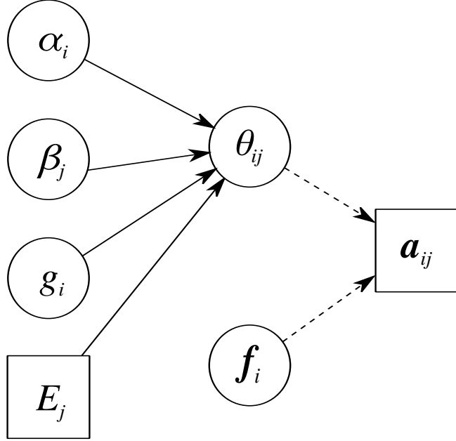
Figure 1: Directed Acyclic Graph (DAG) of the model. Squared nodes denote known quantities ( E for environmental data, and A for genetic marker data). Circled nodes denote unknown parameters. Plain arrows stand for deterministic relationships, and dashed arrows stand for stochastic relationships.
