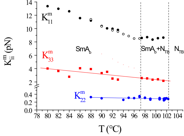
Figure 14. Temperature dependence of all three elastic moduli for the m -director distortion in the intercalated SmA b phase of the BP12 mixture.
