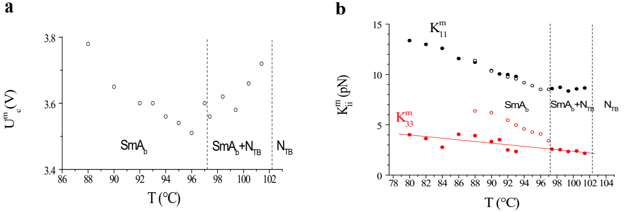
Figure 9. Temperature dependences of the Fréedericksz threshold U_c^m (a) and the elastic constants K_{11}^m and K_{33}^m (b) obtained by fitting the C(U) curves (in the monophasic SmA_b range of the BP12 mixture [16], open symbols) and the optical retardation (solid symbols, discussed below) with the theoretical model. The solid line is a linear interpolation of the K_{33}^m data used for calculation of K_{22}^m .
