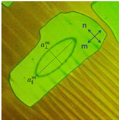
Figure 5. Biphasic \text{SmA}_b/\text{NTB} sample at T = 102.0^\circ\text{C} under electric field ( U = 5\text{ V} > U_c^m , f = 6\text{ kHz} ). The BFrTr takes place in the \text{SmA}_b regions (green). The blue double-headed arrows show the orientation of the \mathbf{n} - and \mathbf{m} -directors of the \text{SmA}_b phase. The elliptically shaped DW that separates one of the twin domains from the other is clearly
