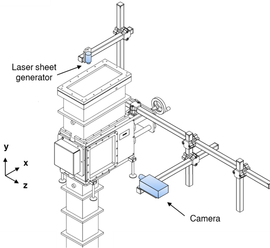
Figure 3 – PIV setup.
