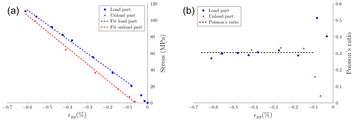
Fig. 4 Mechanical parameter for sample D8. (a) Stress vs strain curve, with the loading in blue and the unloading in red. Dashed lines represent linear fits, excluding the low-strain non-linear response. (b) Poisson's ratio vs strain, with the loading in blue and the unloading in red. The dashed line represents the fit with a constant, excluding the low-strain non-linear response
