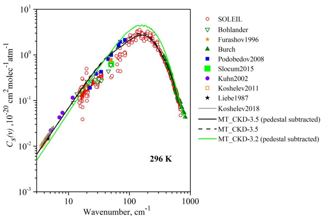
Fig. 1 (analogue of Fig.1 of Paper I). Self-continuum at 296 K: red circles (SOLEIL measurements) [4,9,10], green triangles [7,11], blue squares [12], black star [13], green empty triangles (measurements of R.A. Bohlander) [7], light green square [14], violet circles [15], orange empty squares [16], orange star [17], grey curve [18], green curve (MT_CKD-3.2 model) [2], and dashed and solid black curves are the MT_CKD-3.5 model [2] with and without “the pedestal” (see the text for details), respectively.
