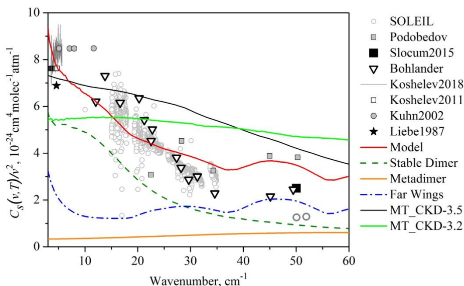
Fig. 3 (analogue of Fig.4 of Paper I). Continuum spectral function: grey empty circles(SOLEIL measurements) [9, 10], black empty triangles [11], grey squares [12], grey curve [18], grey empty squares [16], grey filled circles [15], grey star [17], green dash curve (stable dimer model), orange solid curve (metastable dimer model), blue dash-dot curve (far wings), red solid curve (continuum model obtained as a sum of true bound metastable dimers, and far-wings contributions simulated by in [1]), green curve (MT_CKD-3.2 model) [2], and black thin curve (MT_CKD-3.5 model).
