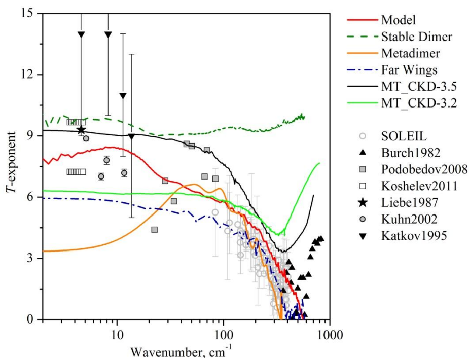
Fig. 2 (analogue of Fig.3 of Paper I). Self-continuum temperature exponent: grey empty circles (SOLEIL measurements) [4], black triangles [7, 11], grey squares [12], black star:[13], grey empty squares [16], black circles [15], black inverted triangles [5], red solid curve (continuum model obtained as a sum of true bound metastable dimers, and far-wings contributions simulated by in [1]), green dash curve (stable dimer) [19], orange solid curve (metastable dimer model), blue dash-dot curve (far wings model), green curve (MT_CKD-3.2 model) [2], and black solid curve (MT_CKD-3.5 model) [2].
