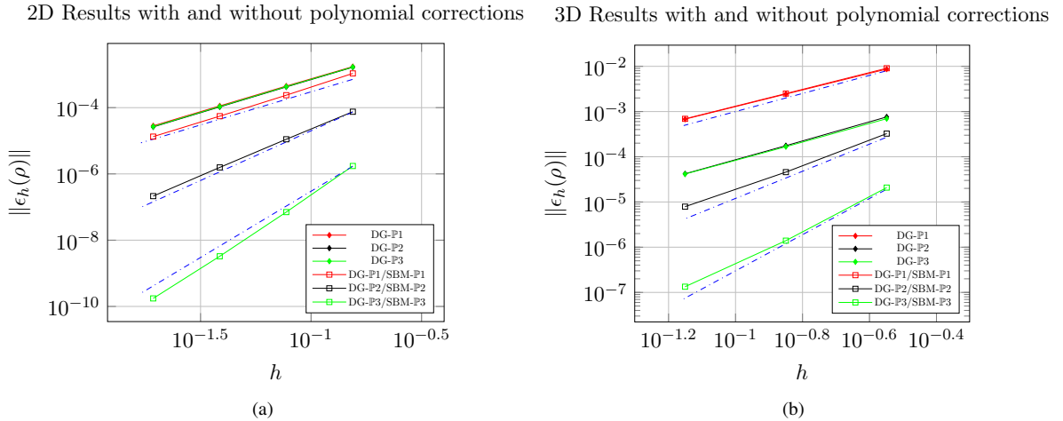
Figure 9: Manufactured solution (2D/3D): results obtained with and without the SBM correction.
