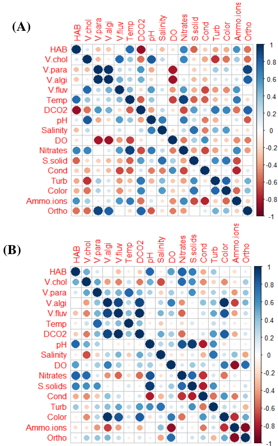
Figure 6. Corrogram for studied parameters at the landing stages of Youpwe 1 (A) and Youpwe 2 (B), correlations shown by color and intensity of shading.
