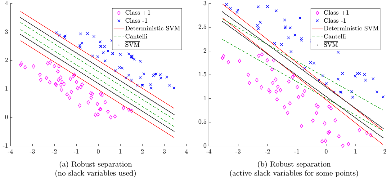
Figure 4: Two-dimensions SVM with \tau = 0.02 , M = 100 , C = 100 .
