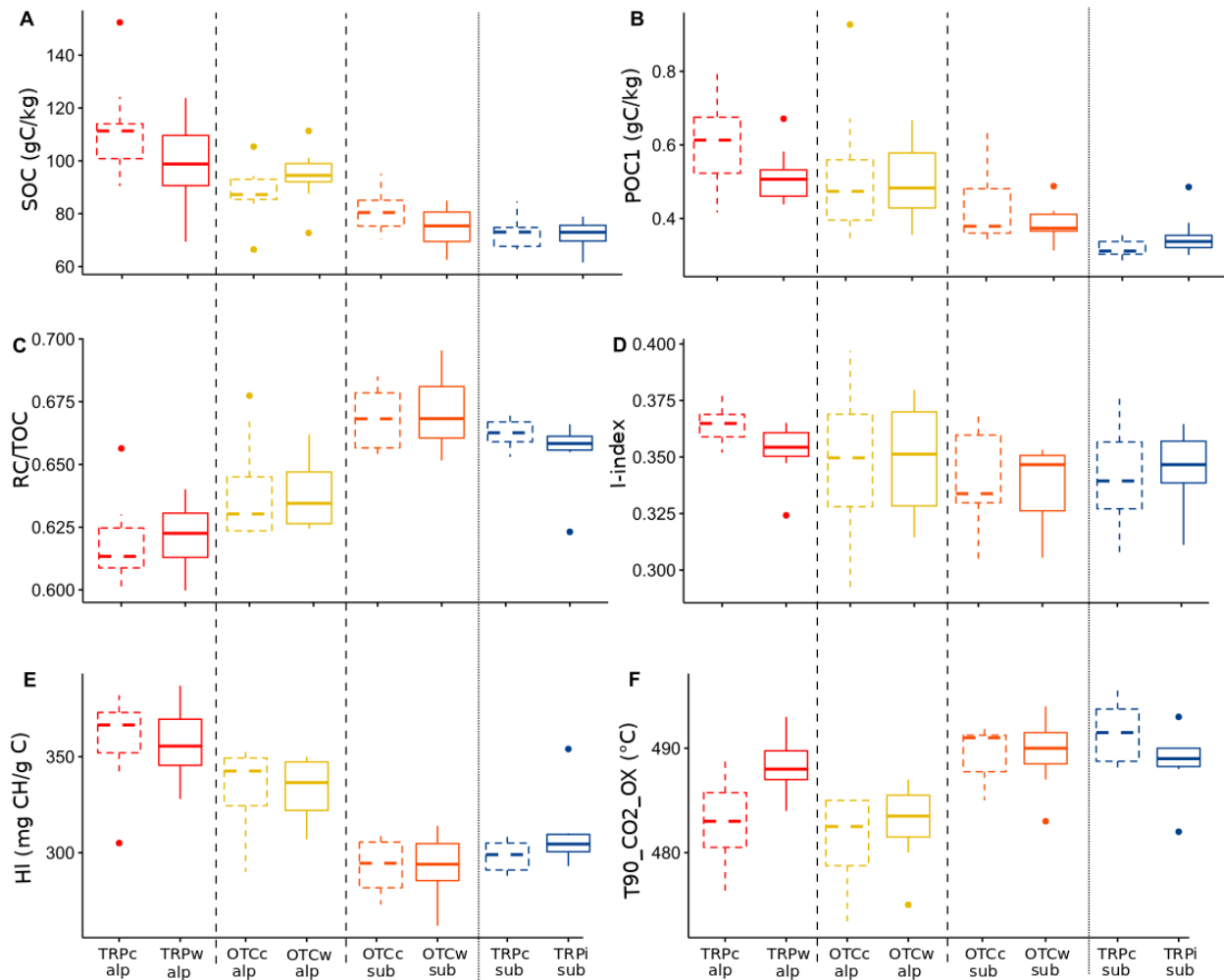
322 323 324 Figure 2: Treatments effect comparisons between control soils (dashed lines) and treated soils 325 (full lines) on (a) SOC content, (b) POC1 content, (c) RC/TOC ratio, (d) I-Index, (e) HI, (f) 326 T 90 _CO 2 _OX parameter. With TRP: transplant, OTC: open-top chamber, c/w/i: 327 control/warmed/cooled, alp: alpine site, sub: subalpine site.
