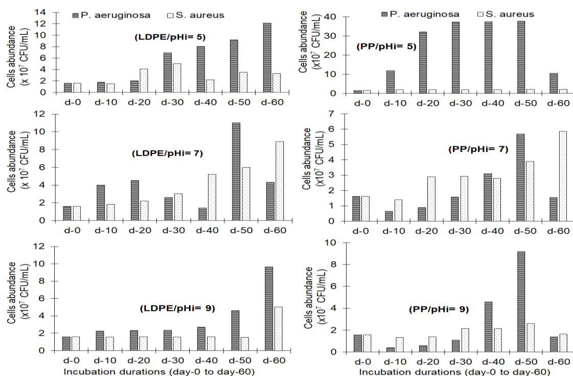
Fig. 4. Temporal variation of the of P. aeruginosa and S. aureus abundance in the presence of the LDPE and PP fragments and under each pH condition of solutions
