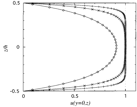
FIG. 3. Normalized velocity profile u(0,z) in the xOz plane for different aspect ratios h/e : analytical results (solid lines) and simulation (symbols) for h/e=2 (○), h/e=5 (×), and h/e=10 (+).
