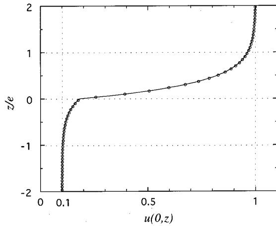
FIG. 4. Velocity profile u(0,z) near the interface between two fluids of viscosity ratio \mu_1/\mu_2=0.1 flowing in a cell of large aspect ratio: analytical results (solid line) and simulation (○). The velocity is normalized by the plane Poiseuille flow maximum velocity of the less viscous fluid Ge^2/(8\mu_1) .
