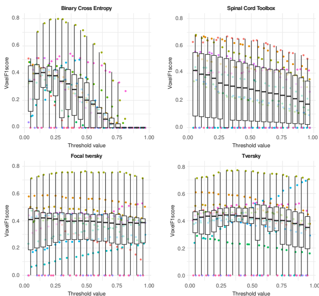
Fig. 2. Boxplots of voxel-wise F1 score for BCE, SCT, Focal Tversky and Tversky losses at each decision threshold value. One point corresponds to one subject.
