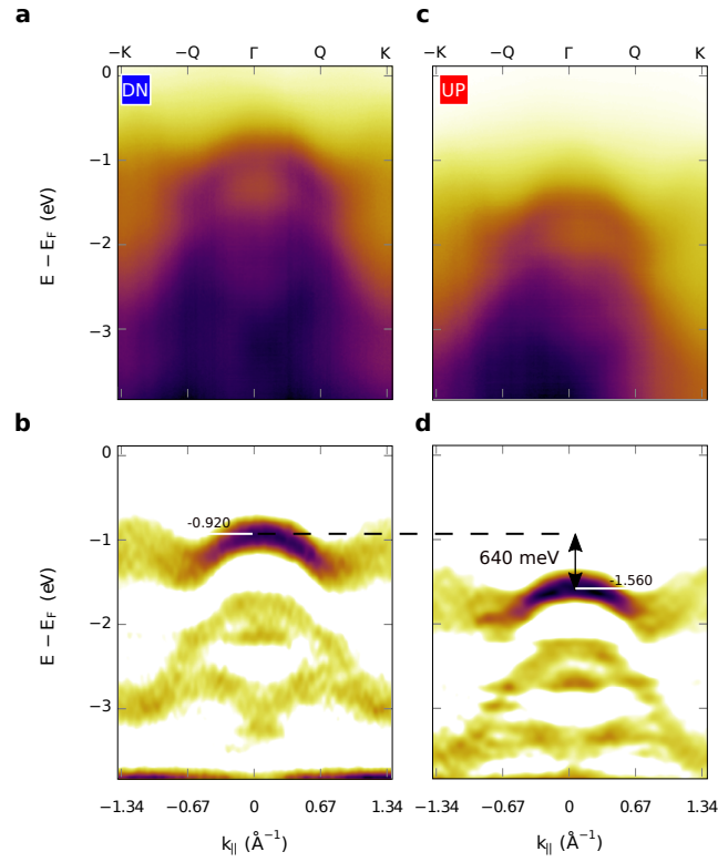
Figure 4: (a) ARPES raw data and (b) second derivative of \Gamma - K slice of the valence band of 2L \text{WSe}_2 on DOWN BFO. (c) ARPES raw data and (d) second derivative of \Gamma - K slice of the valence band of 2L \text{WSe}_2 on UP BFO. The ARPES was measured with h\nu = 50 \text{ eV} and linear horizontal polarization.
