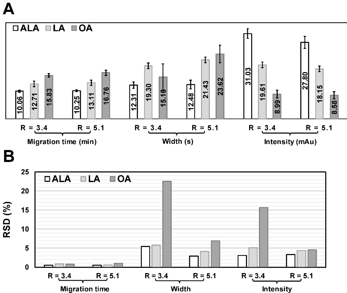
350 Figure 5. A) Effects of R=[\text{NH}_4\text{OH}]/[\text{PFOA}] on the migration times, peak widths, and intensities 351 of three FAs: alpha linolenic acid (ALA), linoleic acid (LA), and oleic acid (LA). A triplicate 352 injection has been performed for each sample. All reported values were averaged. B) Effect 353 of the R ratio on the interdays repeatability ( n = 4 ) of the previous parameters, reported as 354 relative standard deviation (RSD, %).
