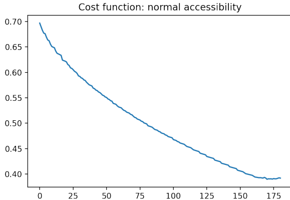
Figure 15: Problem (42): convergence history for the criterion J_{1,\epsilon}(\Sigma) .
