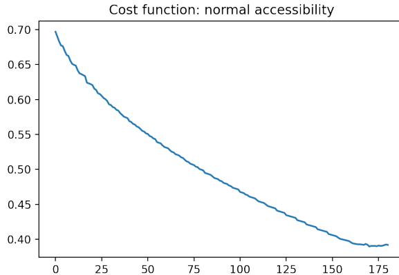
Figure 15: Problem (42): convergence history for the criterion J_{1,\epsilon}(\Sigma) .
