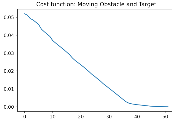
Figure 22: Problem (45): convergence history for the criterion J_{1,\varepsilon}(\Sigma, \Omega_{\text{out}}) .
