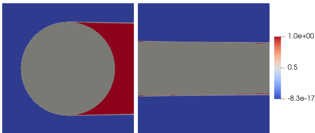
Figure 14: Problem (42): plot of accessibility function h_\varepsilon(d - d_0) for the initial shape (left) and optimized shape (right).
