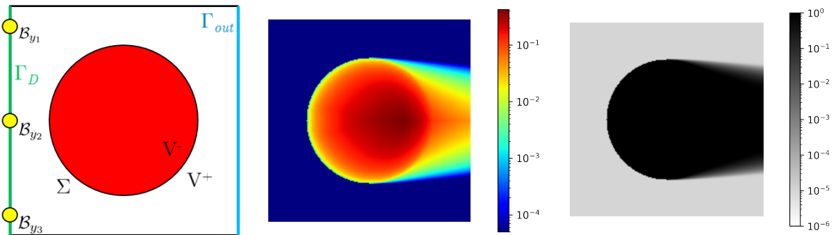
Figure 9: Accessibility of \Gamma_{\text{out}} , measured from three points on \Gamma_D , with a red obstacle (left): fields \min_{i=1,2,3} (d_{y_i} - d_{0,y_i}) (middle) and h_\varepsilon \left( \min_{i=1,2,3} (d_{y_i} - d_{0,y_i}) \right) (right).
