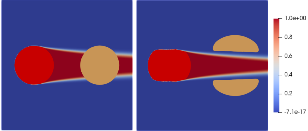
Figure 21: Problem (45): initial shapes (left) and optimized ones (right).
