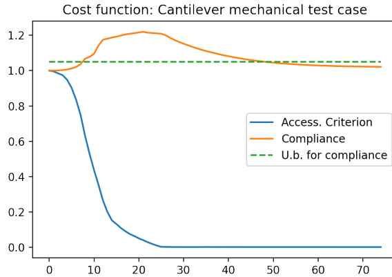
Figure 30: Problem (47): convergence histories for the criterion J_3(\Sigma) (blue) and the compliance (orange) with the upper bound for the compliance (dotted line).
