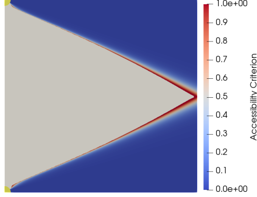
Figure 18: Problem (43): plot of the integrand of J_{2,\epsilon}(\Sigma) for the optimal obstacle obtained with y_1, y_2 placed at the left corners and a volume constraint |\Omega_-| = 0.5 .
