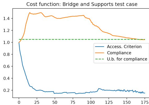
Figure 36: Problem (53): convergence histories for the sum of compliances C(\omega, S) (orange) and the accessibility criterion (54) (blue).
