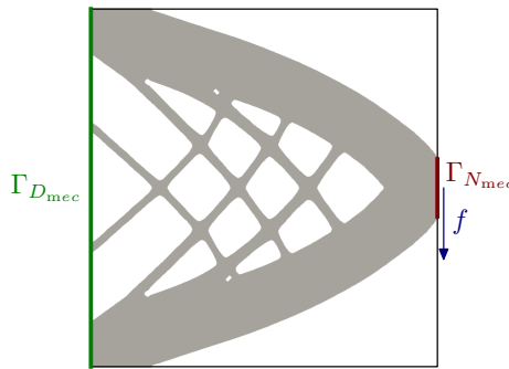
Figure 13: The structure \Omega_- with its boundaries and loads for the elasticity system (35).
