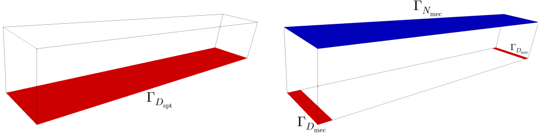
Figure 31: Boundary conditions for the mechanical equations (50) (left) and (51) (right). The load for (50) (left) is a uniform vertical force applied in the structure \omega , while the load for (51) (right) is a uniform vertical force applied on the blue top boundary.
