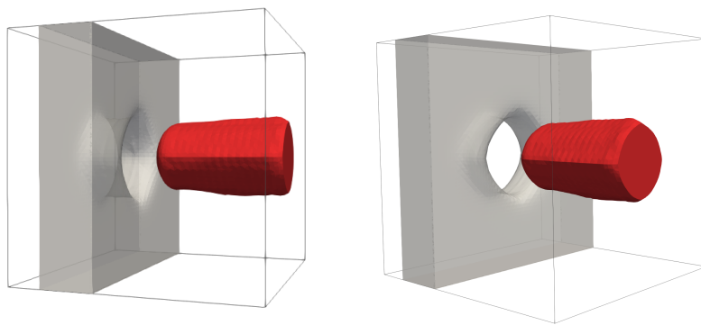
Figure 27: Problem (45) in 3D: two views of the optimized obstacle \Omega_- and target \Omega_{\text{out}} .
