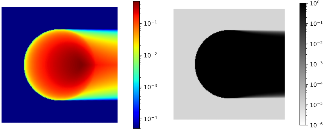
Figure 8: Plots of the fields d - d_0 (left) and h_\varepsilon(d - d_0) (right), showing the non-accessible points on \Gamma_{\text{out}} .
