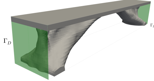
Figure 33: Problem (53): boundary \Gamma_D from which normal accessibility is evaluated.
