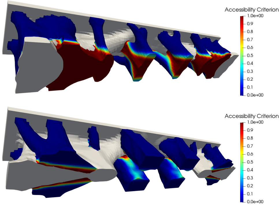
Figure 35: Problem (53): integrand h_\varepsilon(d - d_0) of the accessibility function (54) for the initialization (top) and the optimized design (bottom).
