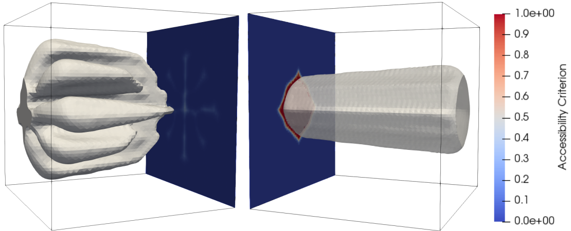
Figure 24: Problem (42) in 3D: optimized obstacle \Omega_- for high diffusion (left) and for low diffusion (right).
