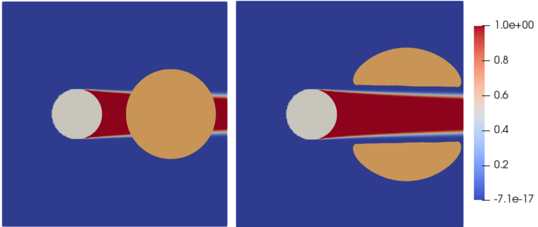
Figure 19: Problem (44): initial shape of the target surface (left) and optimized one (right).
