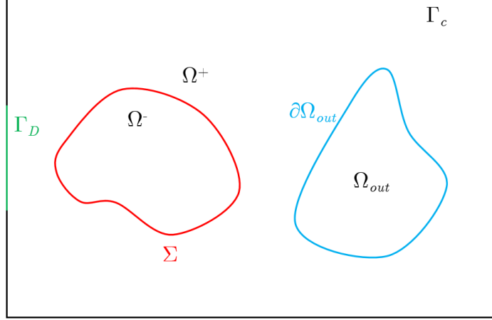
Figure 12: Domain \Omega with a fixed obstacle \Omega_- and a varying subdomain \Omega_{\text{out}} \subset \Omega_+ .
