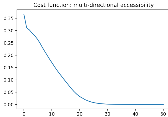
Figure 17: Problem (43): convergence history for the criterion J_{2,\epsilon}(\Sigma) .
