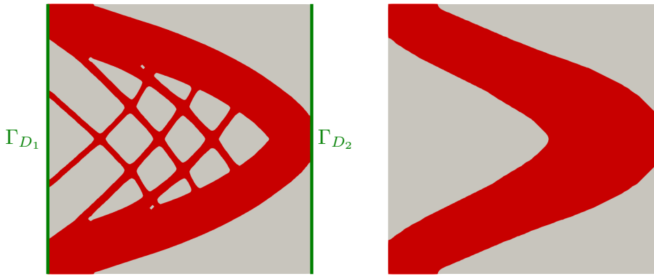
Figure 29: Problem (47): initial reference shape \Omega_-^{\text{ref}} (left) and optimized shape (right).
