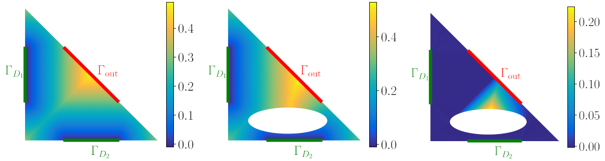
Figure 5: An example of a triangular domain with a white elliptical obstacle \Omega_- , where Definition 2.3 fails to detect a segment connecting \Gamma_D (in green, with two connected components \Gamma_{D_1} and \Gamma_{D_2} ) to \Gamma_{\text{out}} (in red). Distance d_0 (left), distance d (middle), difference d - d_0 (right).
