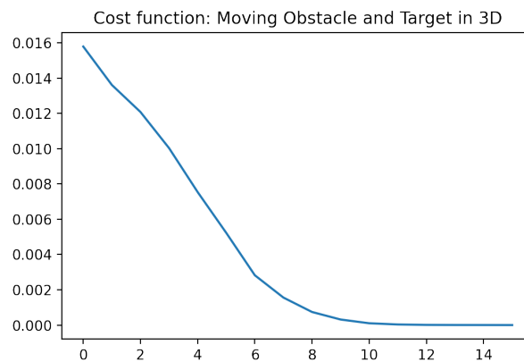
Figure 28: Problem (45) in 3D: convergence history for J_{1,\varepsilon}(\Sigma, \Omega_{\text{out}}) .
