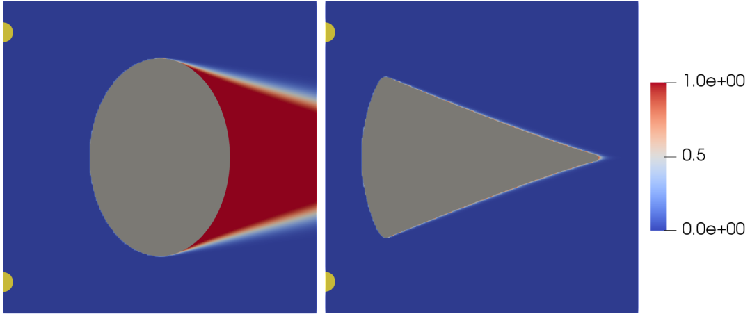
Figure 16: Problem (43): plot of the integrand of J_{2,\epsilon}(\Sigma) for the initial shape (left) and final shape (right).
