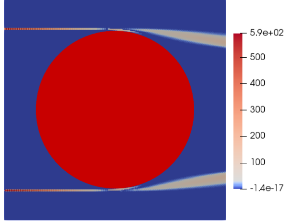
Figure 11: Integrand of the shape derivative (21) for J_{1,\varepsilon}(\Sigma) and a circular obstacle.
