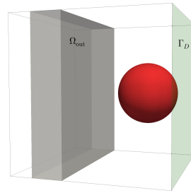
Figure 26: Problem (45) in 3D: initial obstacle \Omega_- (in red) and target \Omega_{\text{out}} (in grey).
