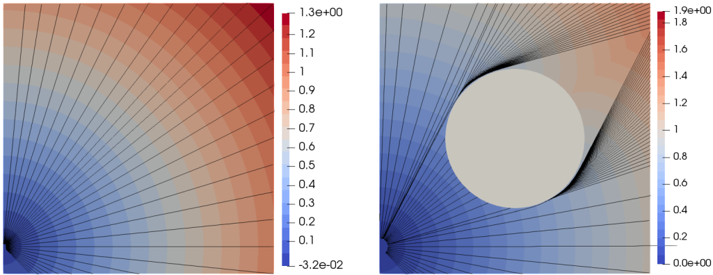
Figure 3: Streamlines or rays of d_{0,y_i} (left, without obstacle) and d_{y_i} (right, with obstacle) issued from the yellow ball \mathcal{B}_{y_i} .
