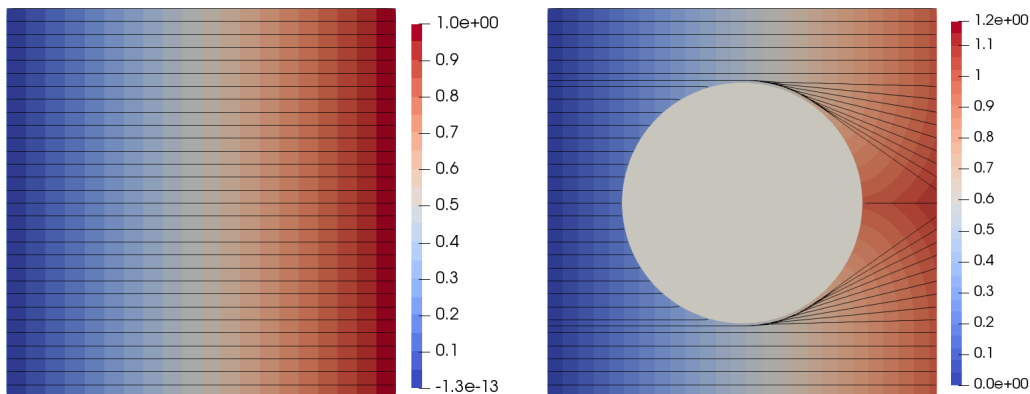
Figure 4: Streamlines or rays of d_0 (left, without obstacle) and d (right, with obstacle) issued from the left side \Gamma_D .
