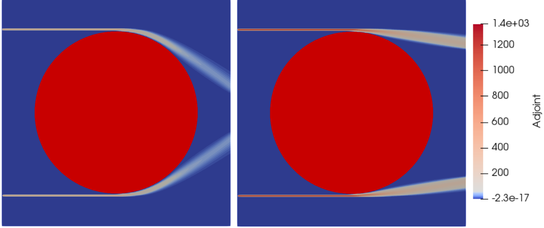
Figure 10: Adjoint state p , solution of (20) for a circular obstacle and J_1(\Sigma) (left) or J_{1,\epsilon}(\Sigma) (right).
