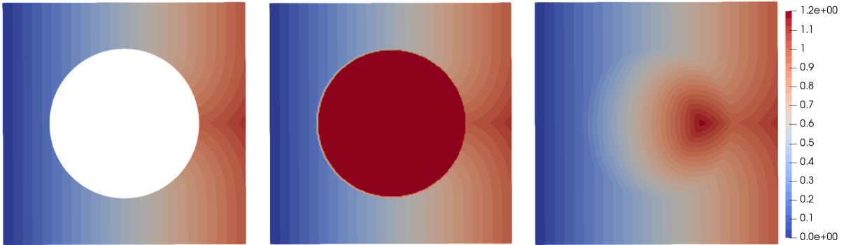
Figure 7: Solution of (7) computed in \Omega_+ only (left), in the complete domain \Omega with V_- = 0.001 (middle) and with V_- = 0.5 (right). In all cases V_+ = 1 .
