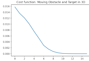
Figure 27: Problem (45) in 3D: convergence history for J_{1,\epsilon}(\Sigma, \Omega_{\text{out}}) .
