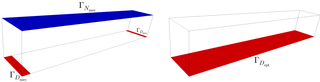
Figure 30: Boundary conditions for the mechanical equations (51) (left) and (50) (right)
