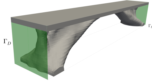
Figure 32: Problem (53): boundary \Gamma_D from which normal accessibility is evaluated.
