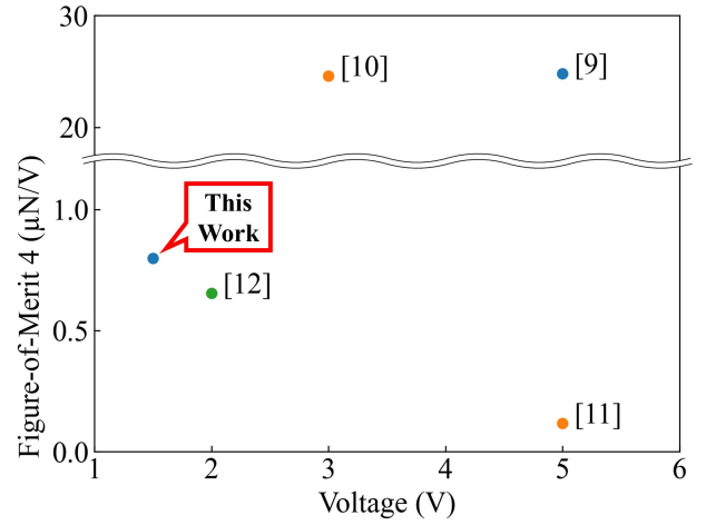
Fig. 12. Figure-of-merit 4 (FoM 4 ) and working voltage.
