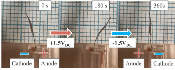
Fig. 3. Bidirectional bending motion of 50b SLIG actuator at \pm 1.5 V DC .
