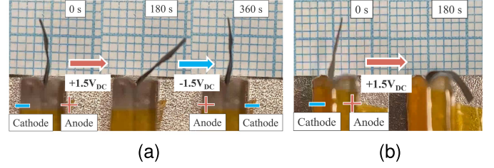
Fig. 4. Measurement of the deformation of the SWIG actuator. (a) Bidirectional bending motion of 50b at \pm 1.5 V DC . Its estimated curvature radius was 5.29 mm by (1). (b) Deformation to the physical limit at the curvature radius of 2 mm. In both figures, the size of the smallest square on the graph paper is 1 mm \times 1 mm.
