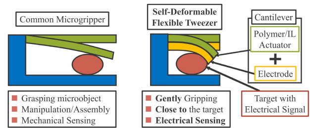
Fig. 1. Common microgripper for micromanipulation and self-deformable close tweezer gripping of a target to detect an electrical signal.
