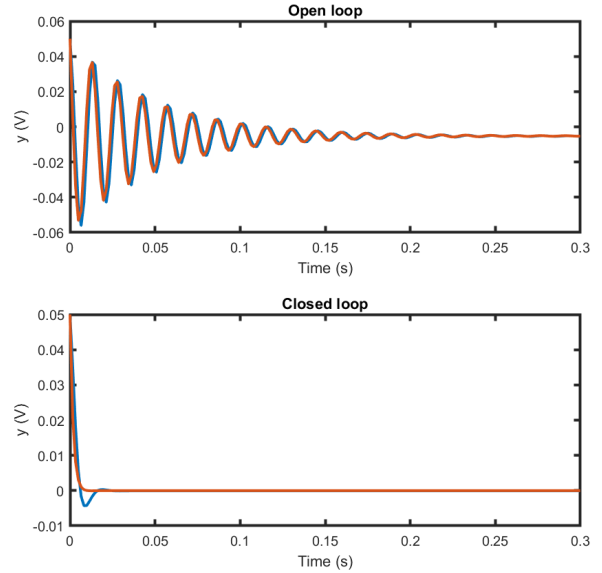
Fig. 3. Comparison of open and closed-loop behavior for model P and M .
