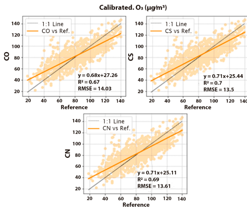
Figure 8. Calibration scatterplots for ozone concentration: Multisensor devices' CO, CS, and CN vs. reference analyzer. Light orange dots represent the individual points sensor—reference, the orange line is the least squares regression line, and the black line represents the x = y line. Units are in \mu\text{g}\cdot\text{m}^{-3} .
