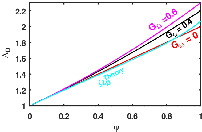
FIG. 15: Different profiles of \Lambda_D(\psi) = 1 + \int \Omega_D(\psi) d\psi , associated with three different \Omega_D(\psi) profiles. Solid red, black and magenta lines are associated with G_\Omega = 0, 0.4 and 0.6 , respectively in Eq. (32). The solid cyan line presents \Lambda_D(\psi) profile for the theoretical expression of \Omega_D(\psi) Eq. (2-3).
