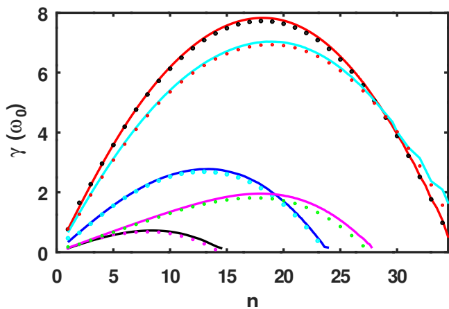
FIG. 17: Growth rate \gamma of different modes n , T_1 with G_T = 3 and different \Omega_D(\psi) profiles, solid red, blue and black lines are for simplified \Omega_D(\psi) expression Eq. (32) with G_\Omega = 0 , G_\Omega = 0.4 and G_\Omega = 0.6 respectively. Solid cyan line: \Omega_D(\psi) theoretical expression Eq. (2-3) with \kappa = 0 , G_T = 3 and solid magenta line: for G_T = 2 and the theoretical expression of \Omega_D(\psi) . The dots are the results from linear TERESA simulations.
